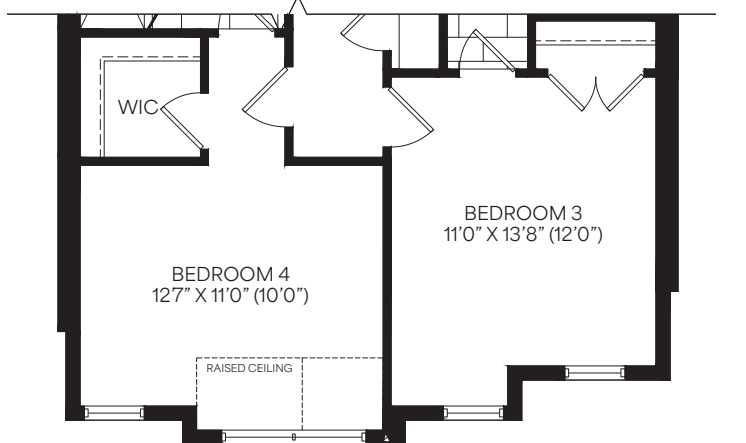
Second Floor Elevation B
