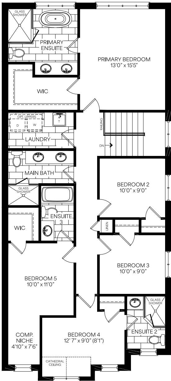
Second Floor Optional 5 Bedroom Plan Elevation A
