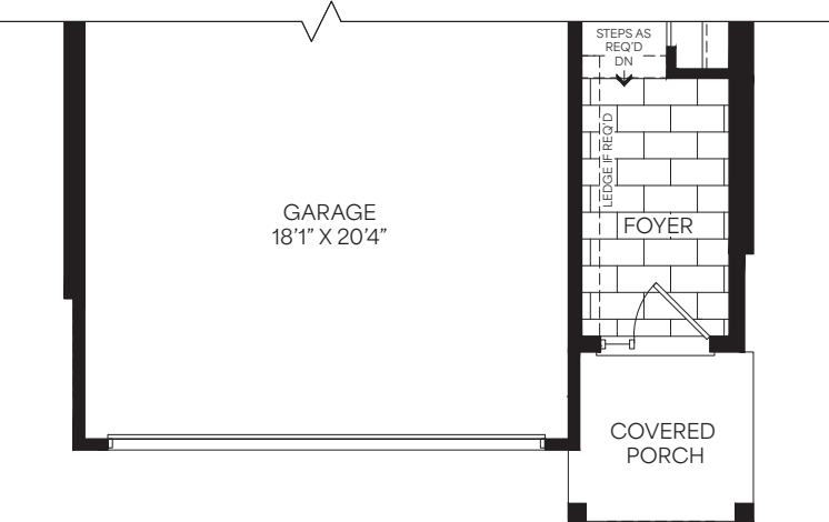
Main Floor Elevation B
