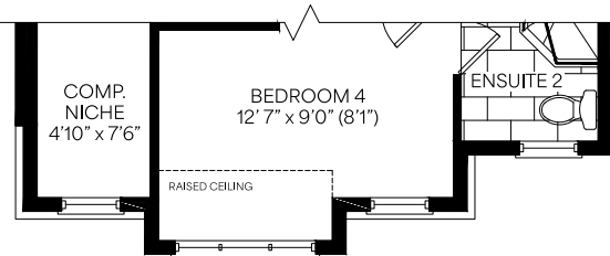
Second Floor Optional 5 Bedroom Plan Elevation C
