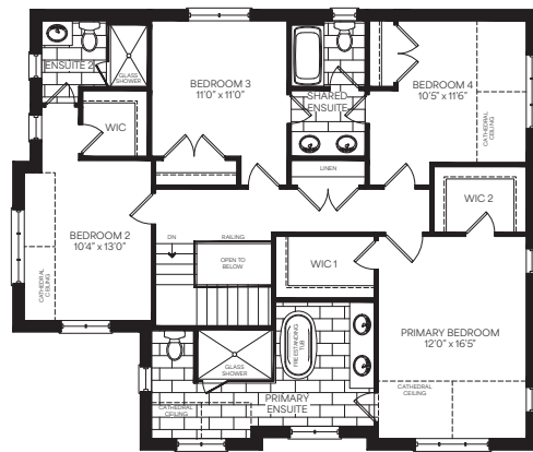
Second Floor Elevation A
