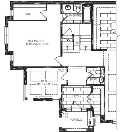
Main Floor Optional In-Law Suite Elevation C
